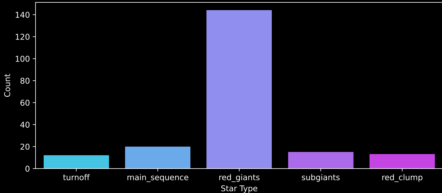
APOGEE DR17 Field: [191+04] Count plot of Star Type
