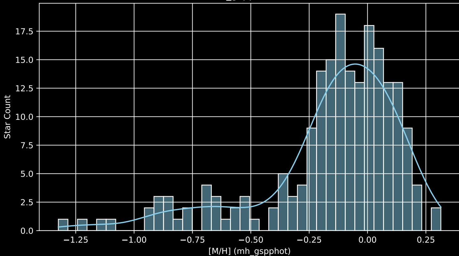
APOGEE DR17 Field: [191+04 [M/H] (mh_gspphot) (n= 202)
