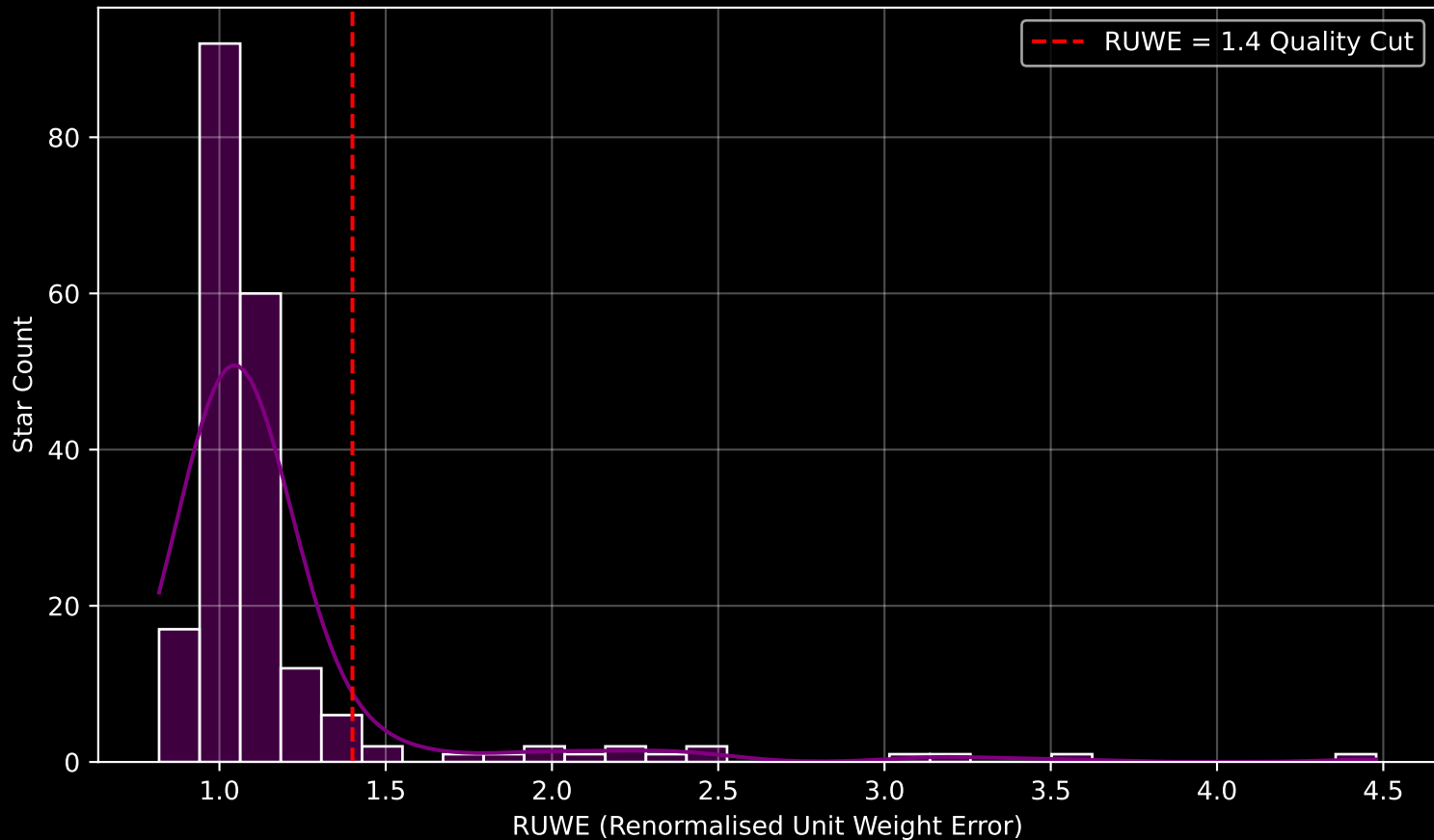
GAPOGEE DR17 Field [191+04] RUWE Distribution (n= 203)
