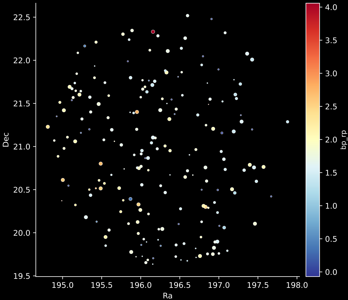
APOGEE DR17 Field: [191+04] Stars: 204
