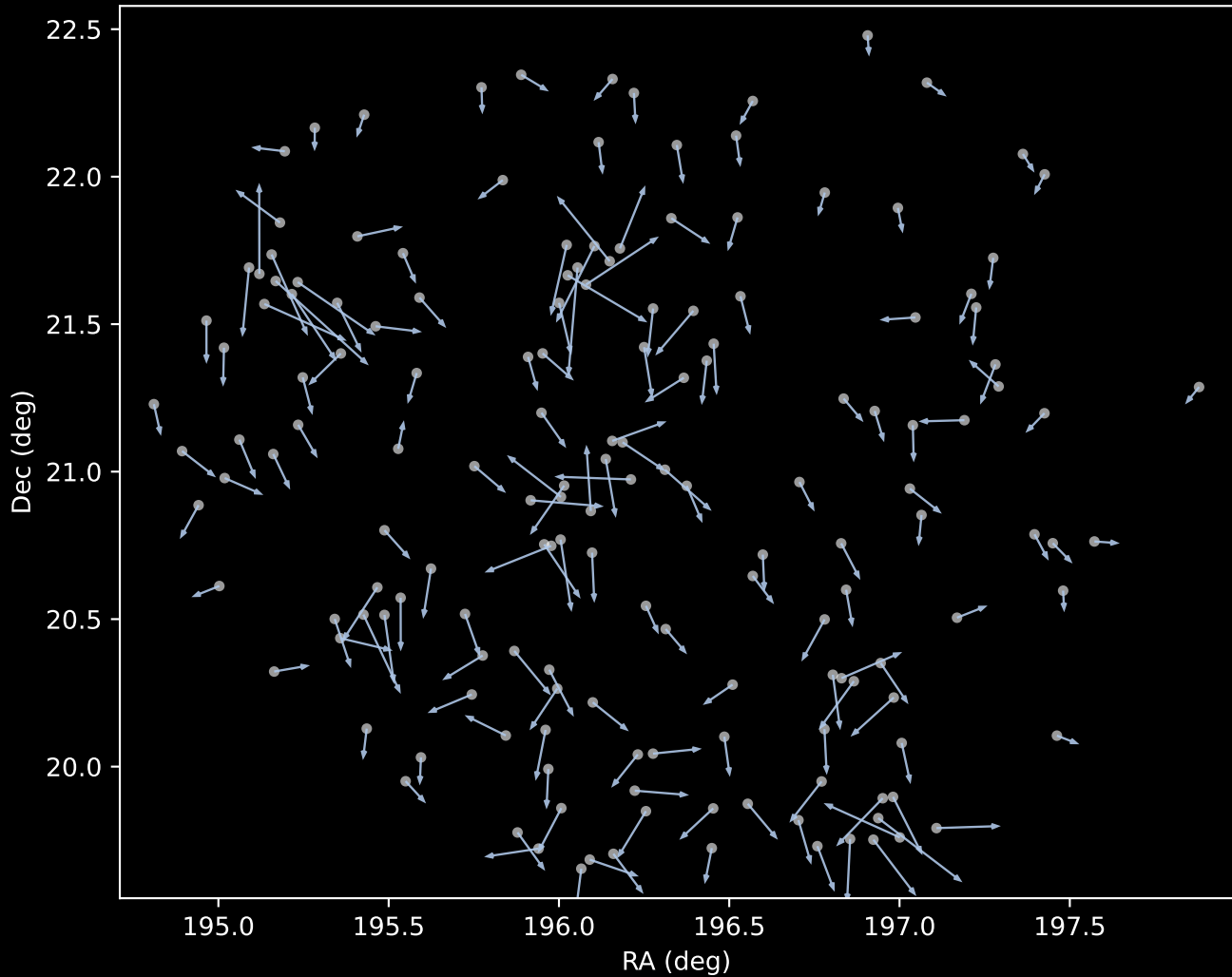
APOGEE DR17 Cluster 1 Proper Motion Vectors (n=162)
