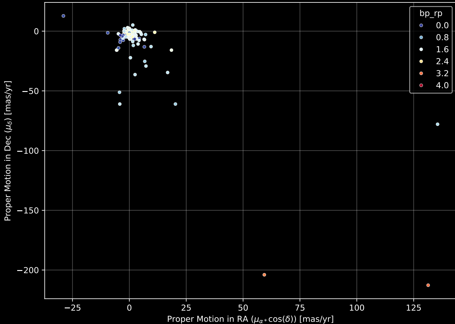
APOGEE DR17 Field: [191+04] Proper Motion Diagram (n = 204)
