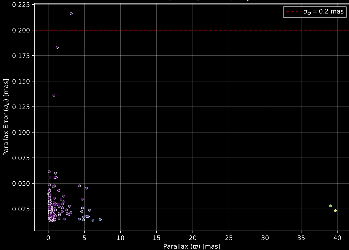
APOGEE DR17 Field: [191+04] Parallax Quality (n= 204)
